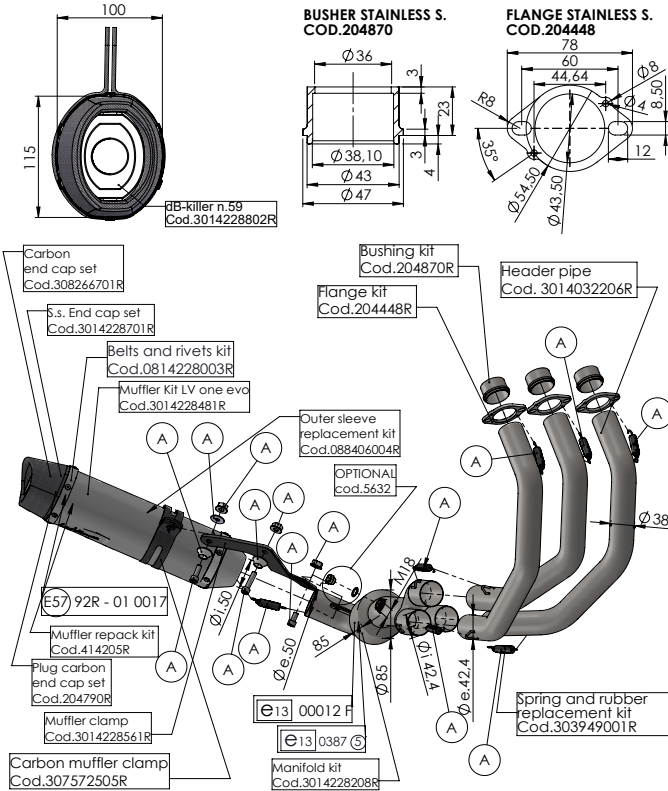
ART. 14228EK SPARE PARTS
