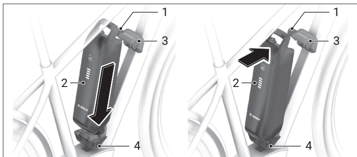
Fig.: 9 Removing and inserting the PowerPack battery
