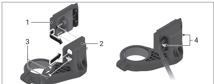
Fig.: 16 Installation of the control computer holder
